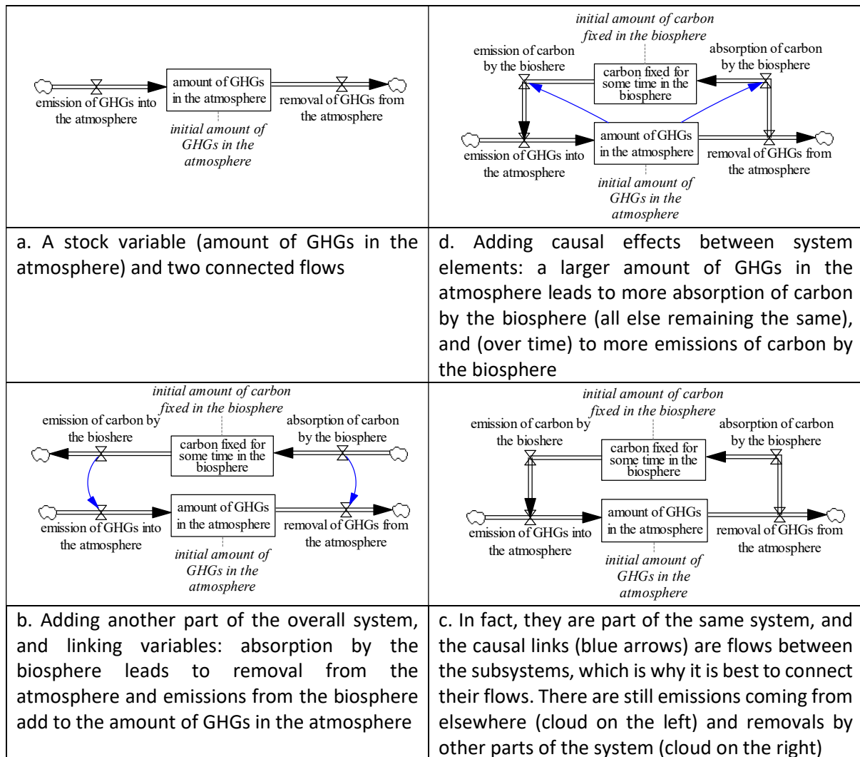
Figure 31: SD model building by building up a Stock-Flow diagram
